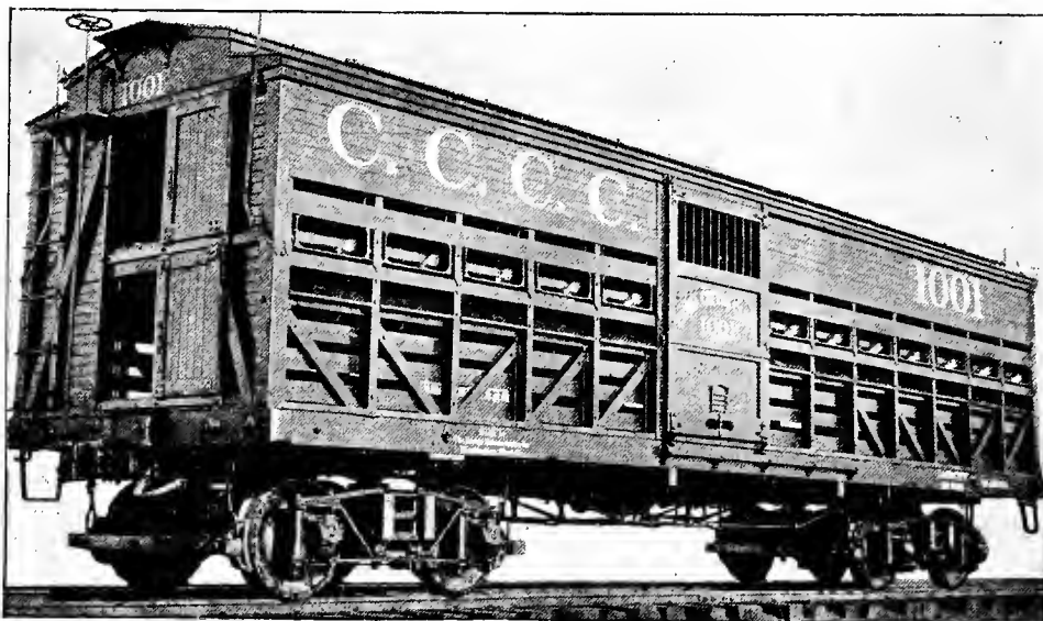
Fig. 40. STOCK CAR FOR CATTLE AND HORSES. CANADA CATTLE CAR COMPANY. Length, 36 ft. Capacity, 60,000 lbs. Weight, 32,900 lbs. Arrangements for Feeding and Watering, End Doors for Loading Lumber and Rails, and Equipped with Air Brakes and Special Swing Motion Trucks. (Details are shown in Figs. 339-364.)
